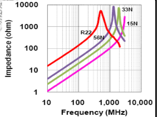
Z vs. Frequency ML160808H Series
