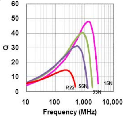
Q vs. Frequency ML160808H Series
