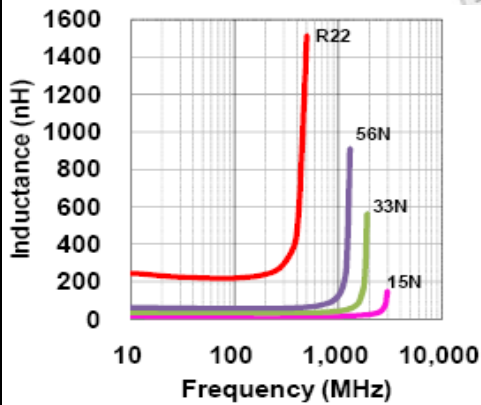
L vs. Frequency ML160808H Series
