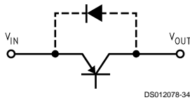
FIGURE 4. LP2980 Reverse Current Path
