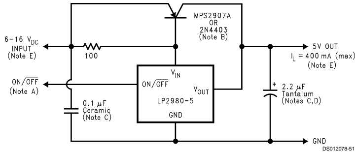
FIGURE 5. 5V/400mA Regulator
