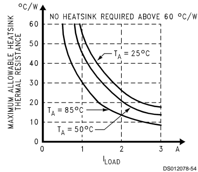
FIGURE 8. Heatsink Thermal Resistance Requirements for Figure 7
