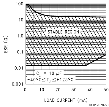
FIGURE 3. 10 \mu\text{F} ESR Range
