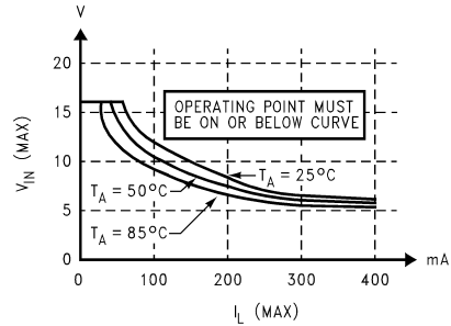
FIGURE 6. Safe Operation Boundary Curves for Figure 5
