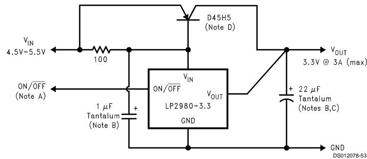
FIGURE 7. 5V to 3.3V @ 3A Converter
