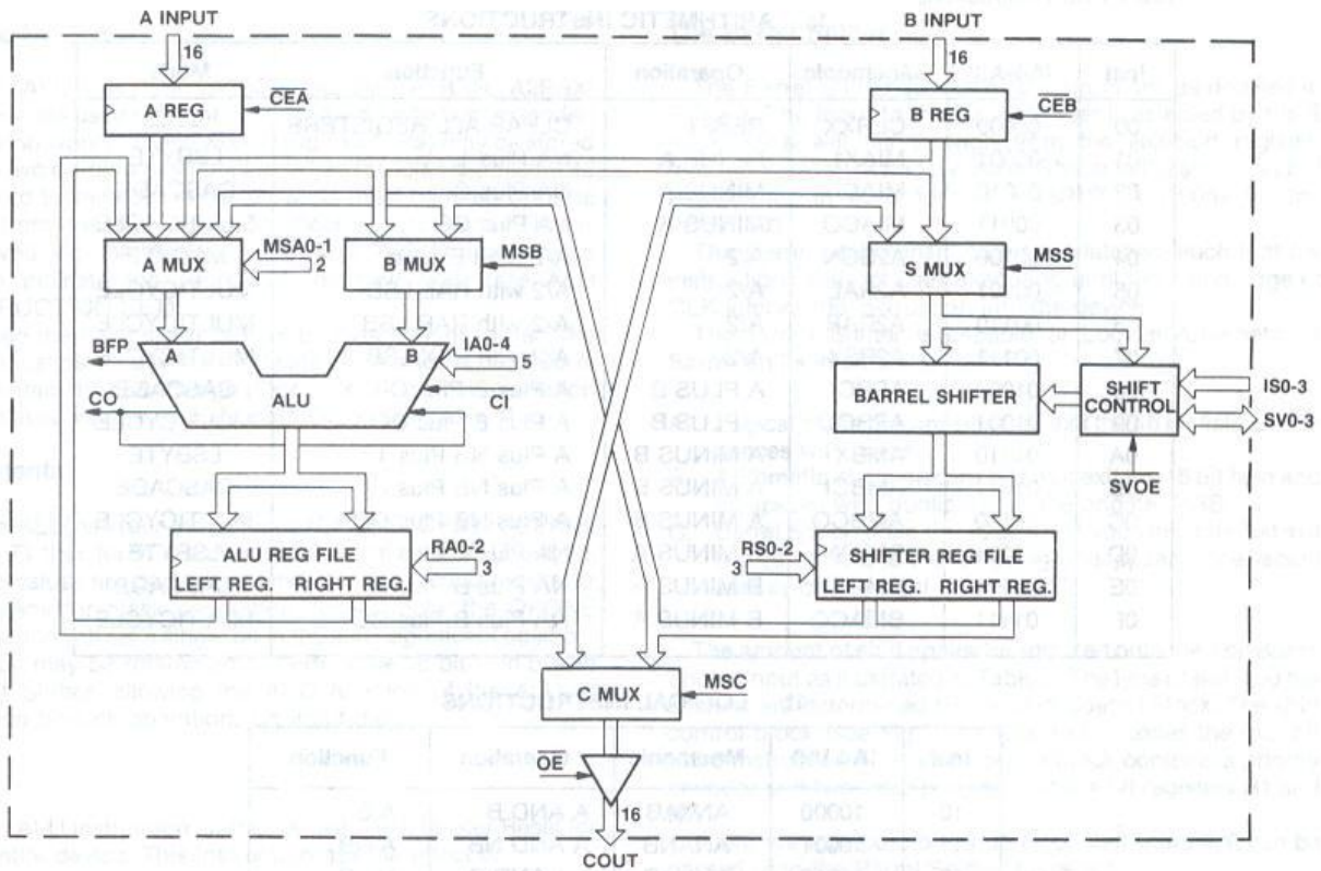
Fig.2 PDSP1601 block diagram
