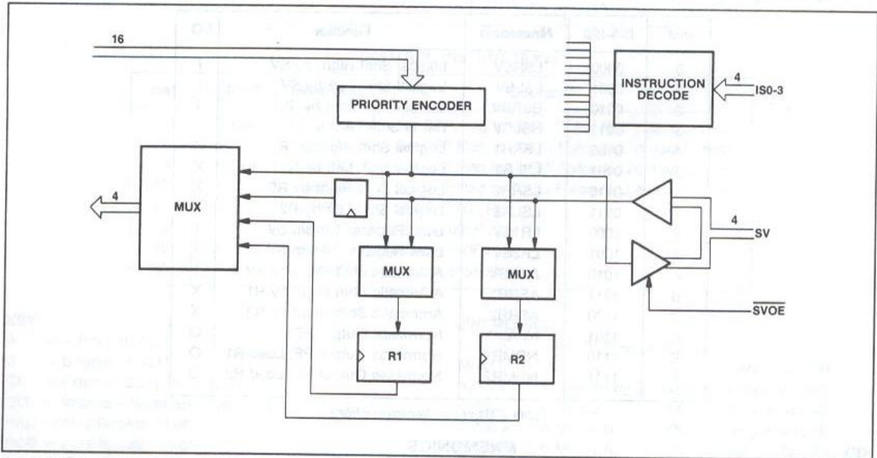
Fig.3 Shift control block
